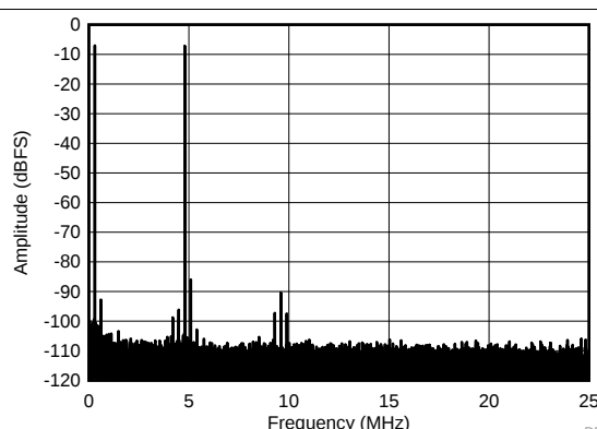
Figure 40. FFT for 450-MHz Input Signal (Dither On)
