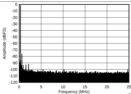
Figure 38. FFT for 270-MHz Input Signal (Dither On)
