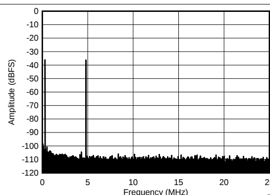
Figure 41. FFT for 450-MHz Input Signal (Dither Off)
