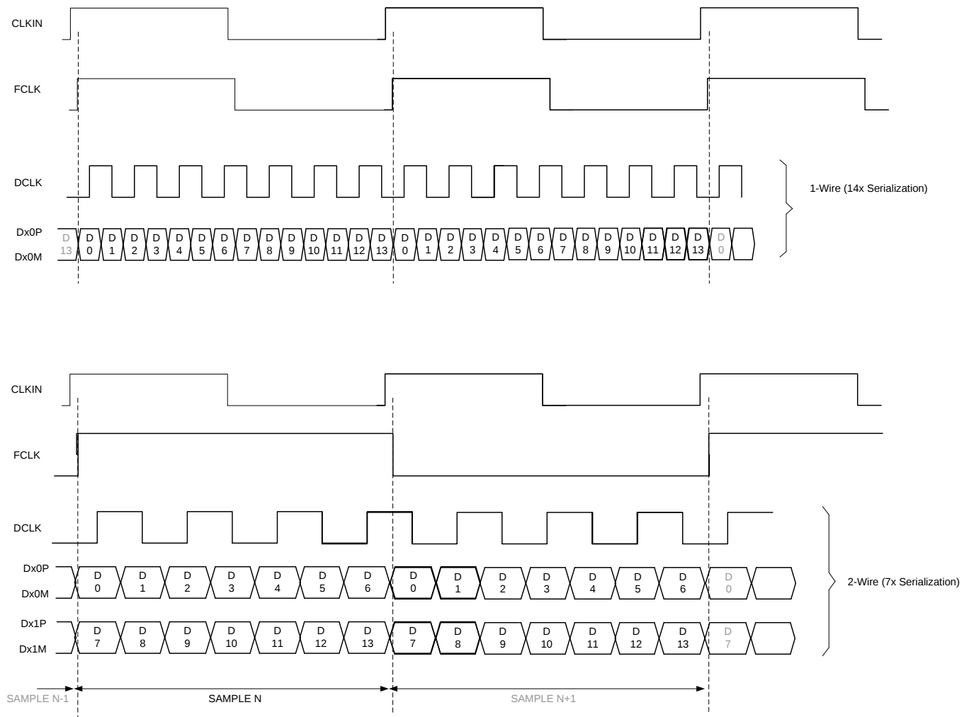
Figure 133. Output Timing Diagram
