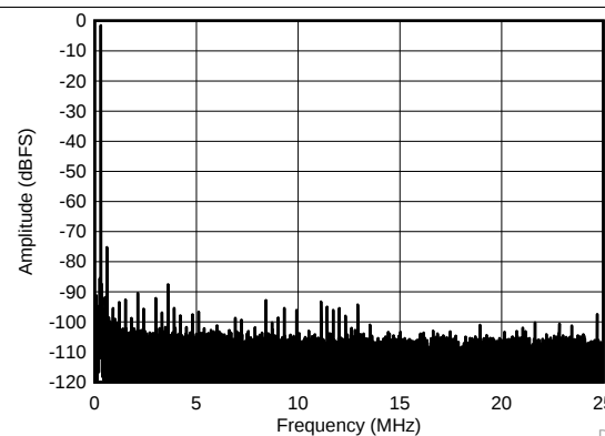
Figure 39. FFT for 270-MHz Input Signal (Dither Off)
